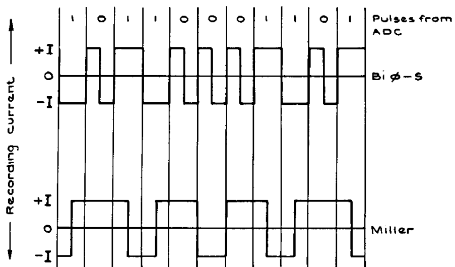
Fig.27 Bi \phi - S and Miller codes
