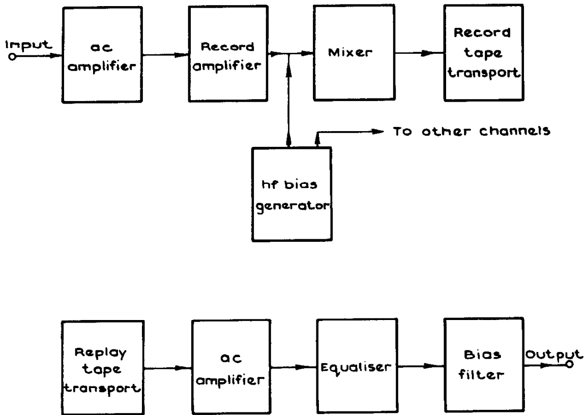
Fig.7 Direct record and replay sub-systems
