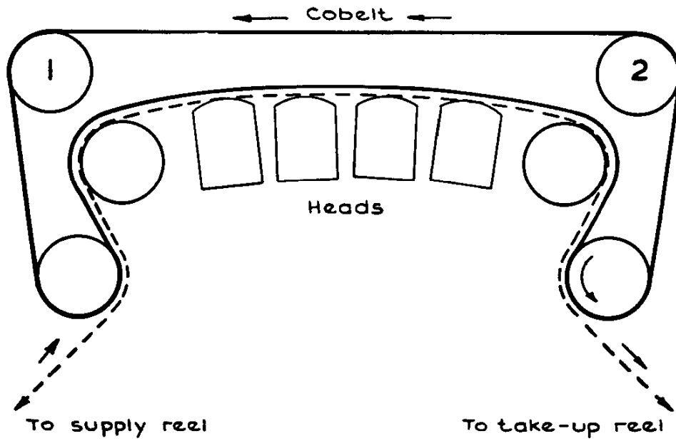
Fig.34 Cobelt drive system
