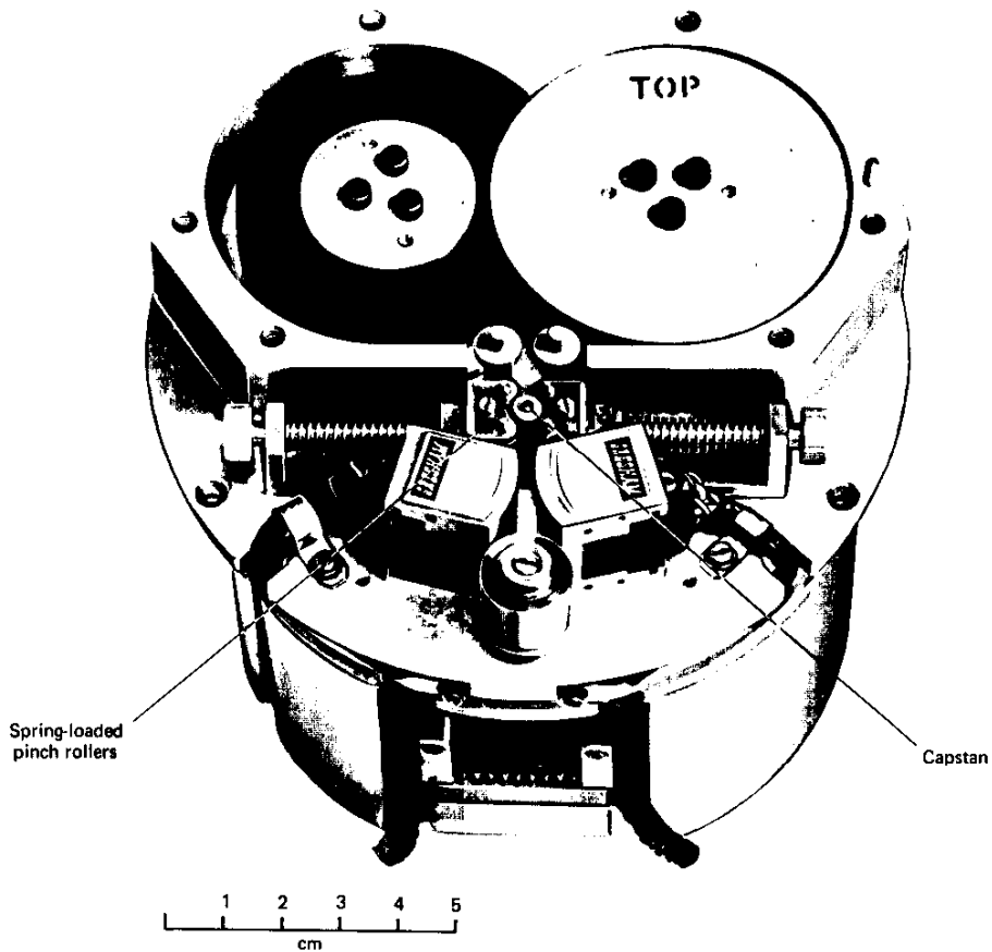
Fig.39 Weapon-borne transport with integral power unit
