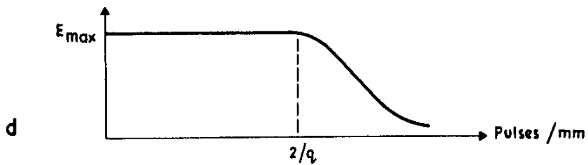
Fig.20 Pulse crowding
