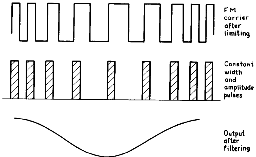
Fig.23 Pulse type FM discriminator
