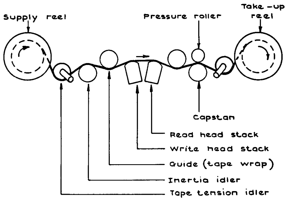
Fig.31 Open-loop drive system
