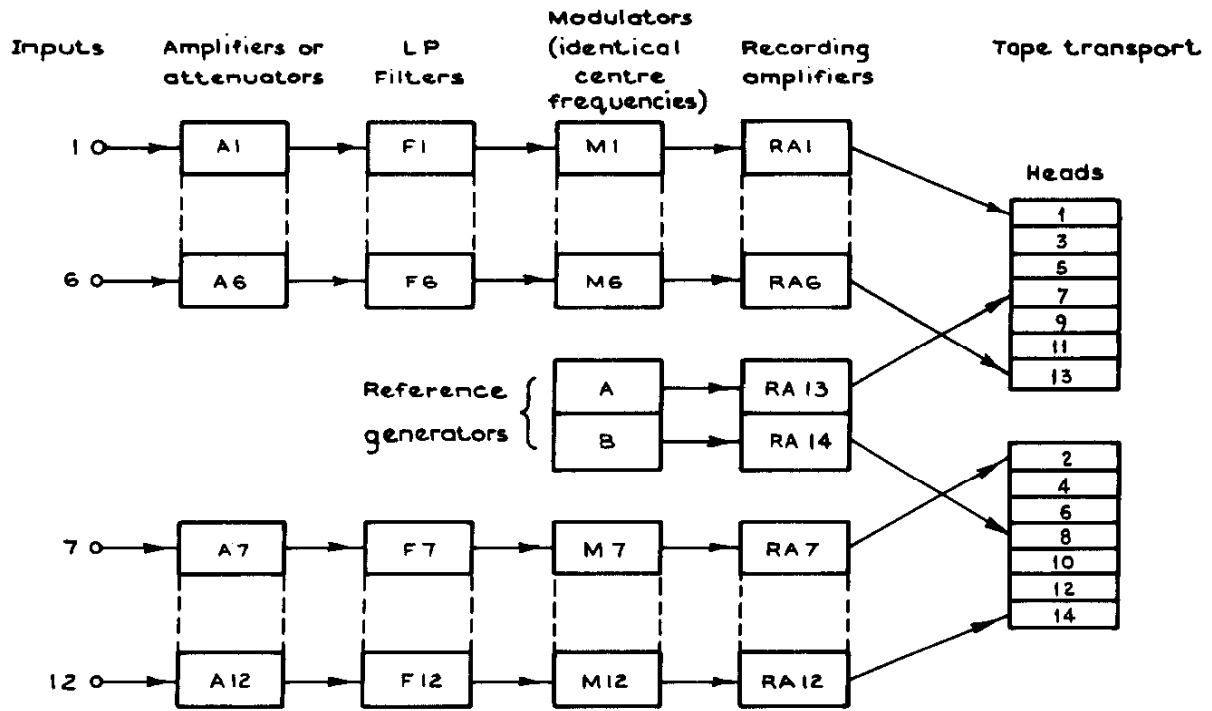
Based on IRIG standard: 7+7 head stacks Fig.3 Single-carrier FM record sub-system
