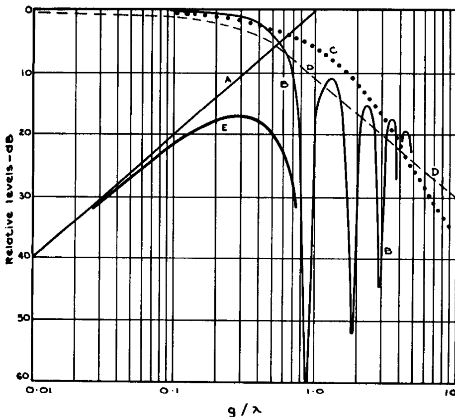
Fig.17 Head/tape relationship for ring-type head
