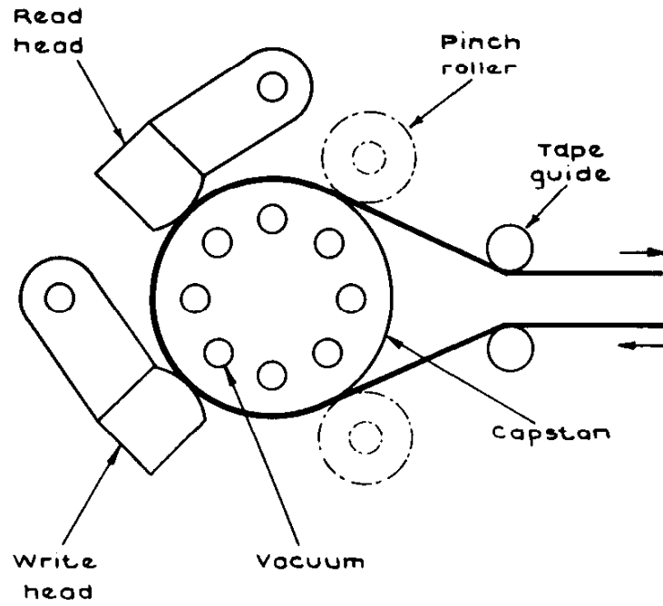
Fig.33 Zero-loop drive system
