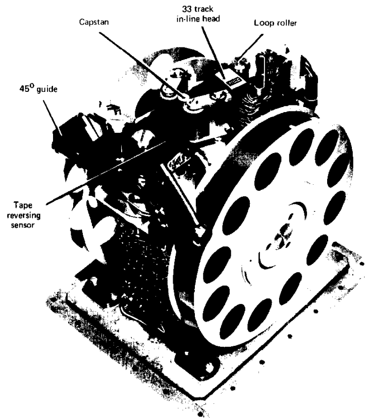
Fig.37 Airborne tape transport with dual capstan drive
