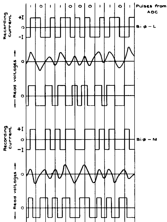
Fig.26 Phase modulation waveforms (Biφ-L and Biφ-M)
