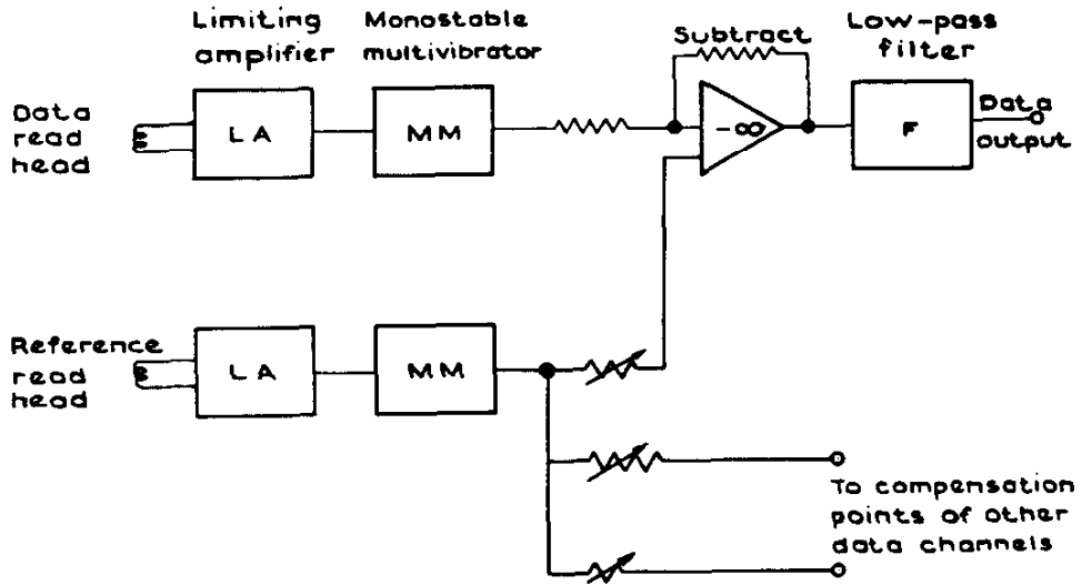
Fig.29 FM demodulation with subtractive compensation
