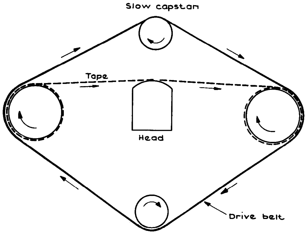
Fig.35 ISO-elastic drive system
