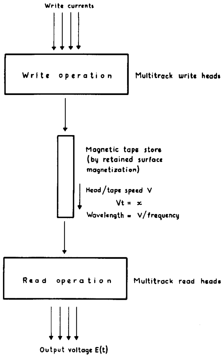
Fig.16 Representation of the magnetic recording process
