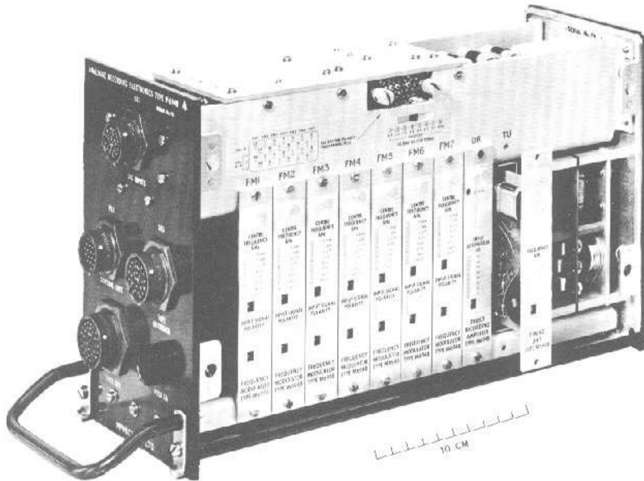
7 FM channels - all speeds (with direct record interrupt facility on 1100) plus reference channel in half AIR short case
