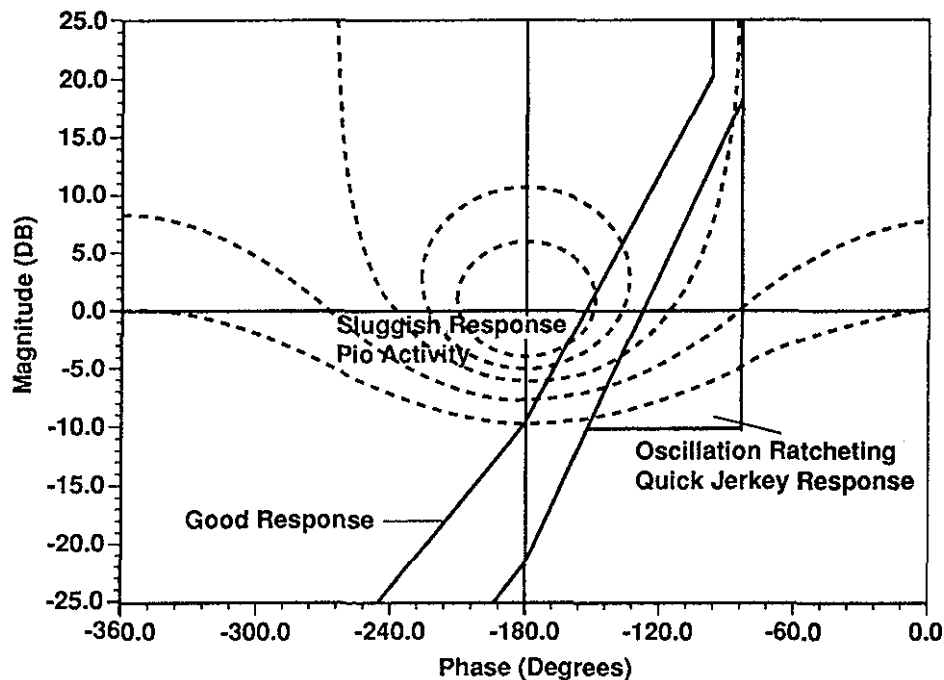
Figure B.1.3 Bank Angle Frequency Response Boundaries for PIO Detection
