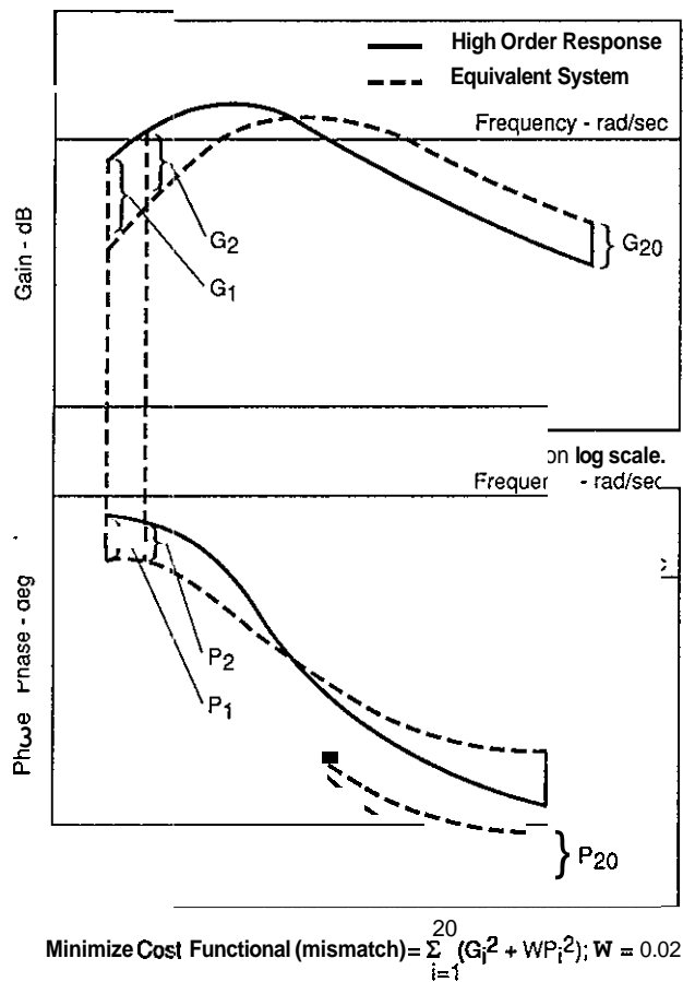
Figure 4.2.1 Optimizing Cost Functional for Equivalent System Determination
