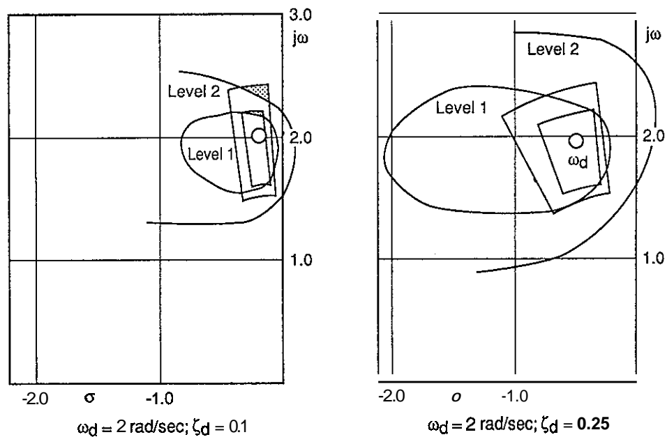
Figure B.1.4 Level 1 and 2 Boundaries Comparison Between MIL-87858 and Northrop Criterion
