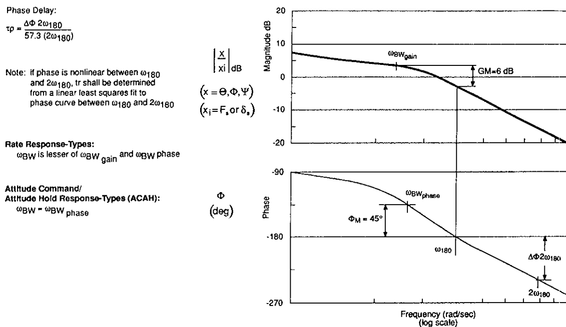
Figure 4.3.1 Definition of Bandwidth and Phase Delay
