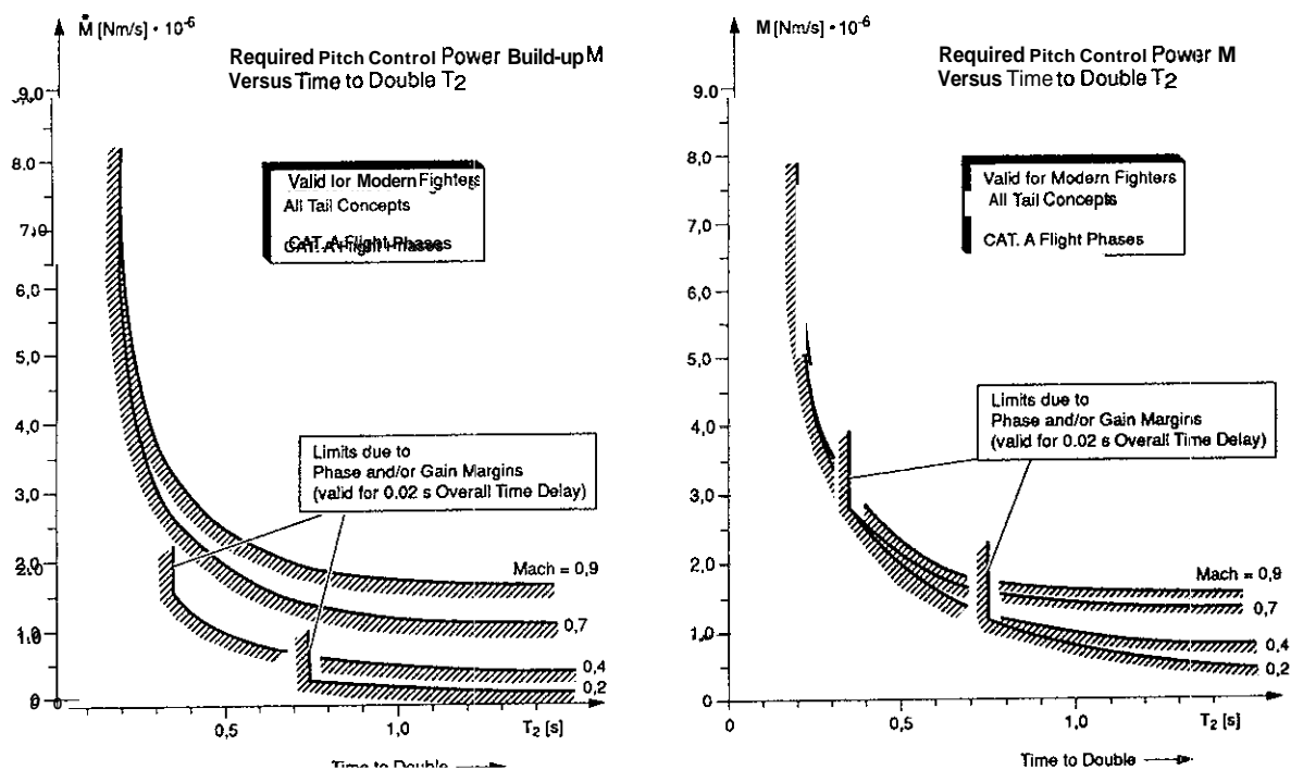
Figure 6.4.3 Criteria for Pitch Control Power
