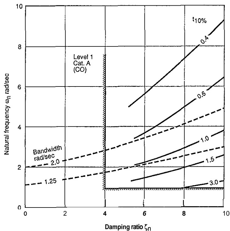
Figure B.1.7 Dutch Roll Characteristics
