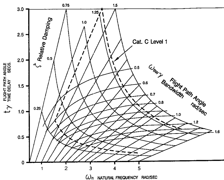
Figure 5.3.1 Transformed Frequency and Damping Boundaries
