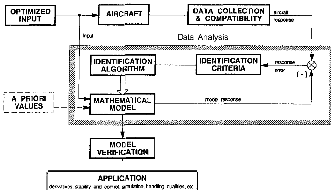
Figure 8.4.1 System Identification Procedure and Utilization
