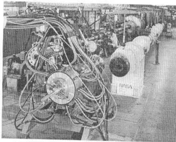
Figure 9. NASA Ames Electric Arc Shock Tube.
