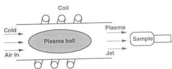
Figure 22. Schematic of VKI Plasmatron.
