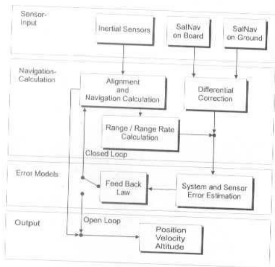
Fig. 5 Schematic of integrated DGPS/INS navigation system used in flight tests
