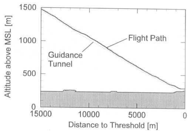
Fig. 20 Flight test results (route B in Fig. 19)
