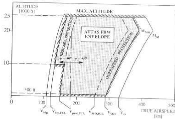
Fig. 8: ATTAS FBW Envelope
