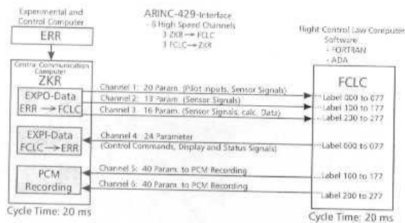
Fig. 10: Communication between ZKR and FCLC
