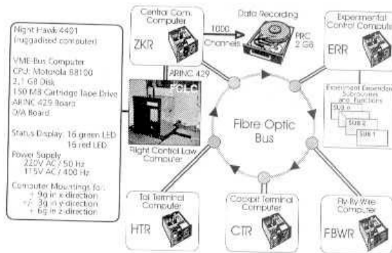
Fig. 9: FCLC Integration into ATTAS Test System
