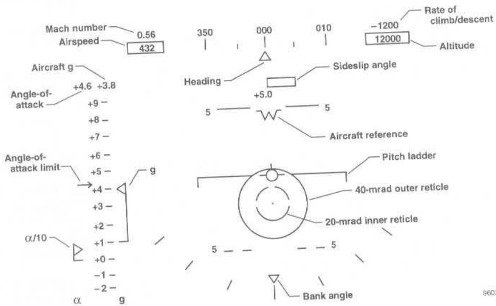
Figure 2. Head-up display symbology.
