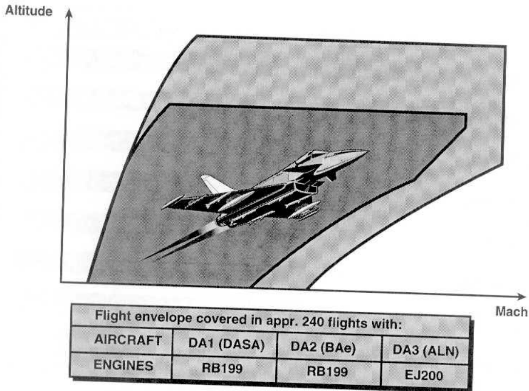
Figure 5: Flight Test Status
