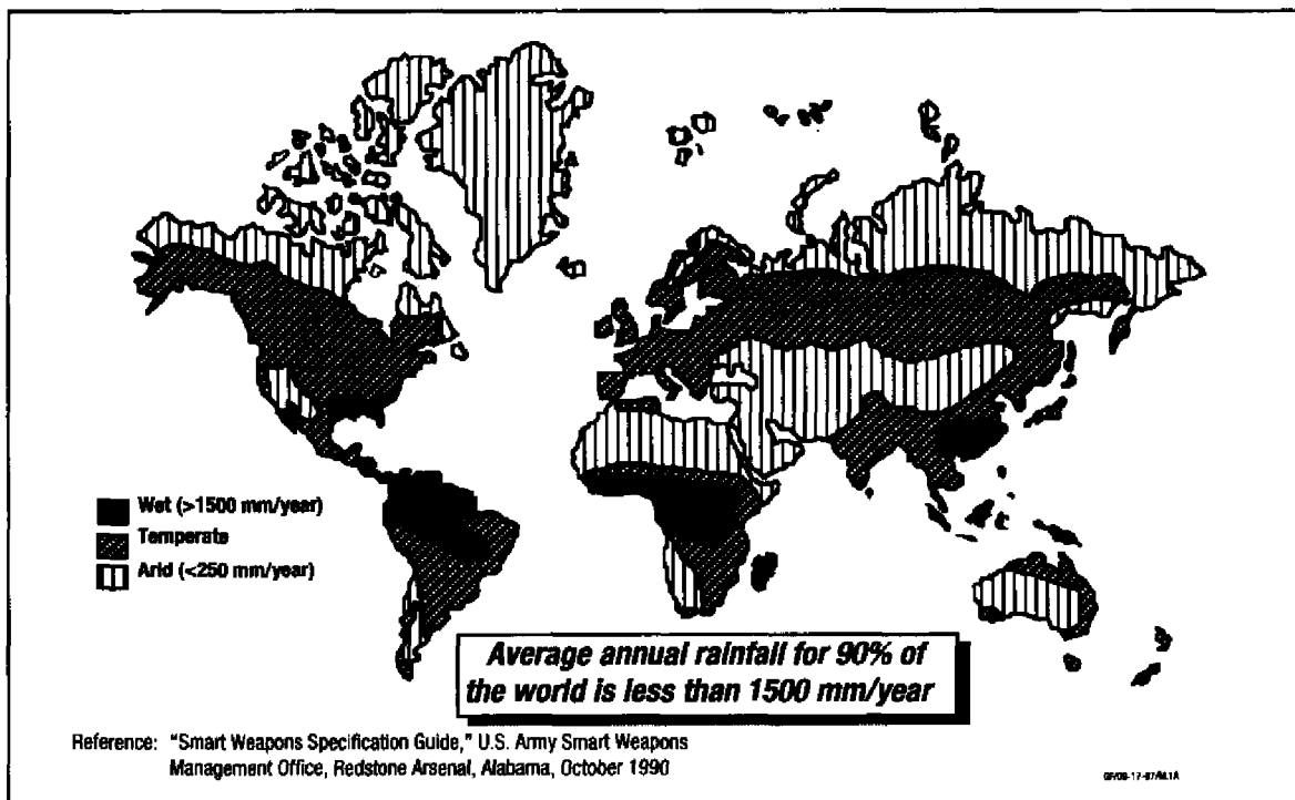
Figure 2. Rain Climatology
