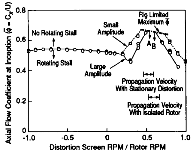
Figure 22: Effect of distortion rotation rate on compressor stall onset [29].
