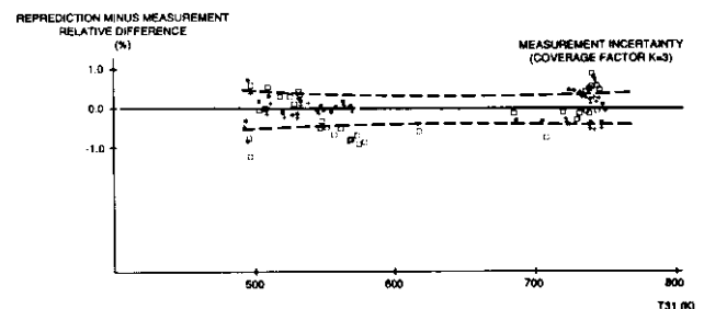
FIGURE 19 - MEASUREMENT - REPRODUCTION COMPARISON - HPC EXIT TEMPERATURE T31
