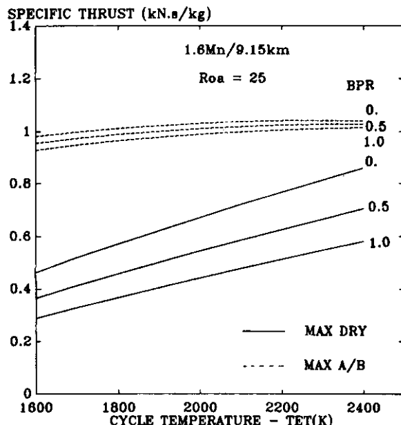
FIG. 27 MILITARY ENGINE SPECIFIC THRUST TRENDS
