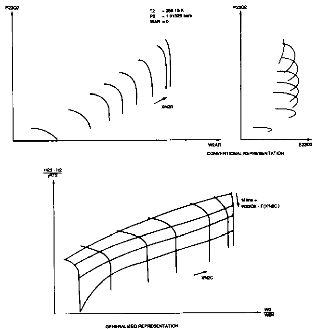
FIGURE 4 - REPRESENTATION OF CHARACTERISTICS OF A LP COMPRESSOR
