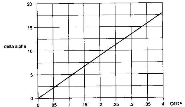
Fig. 21: Turbine Exit Flow Angle Variation Due to Inlet Temperature Distortion
