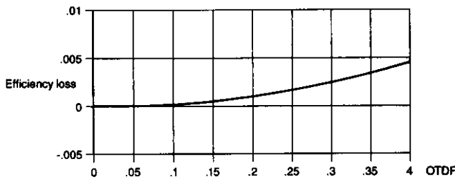
Fig. 20: Efficiency Loss Due to Inlet Temperature Distortion OTDF
