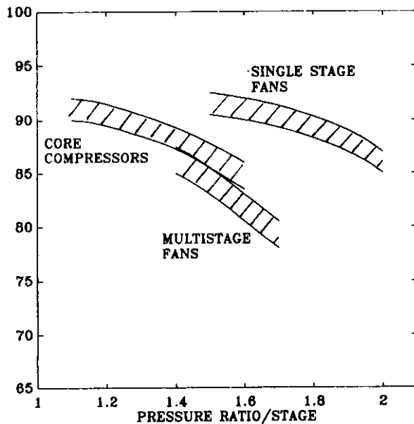
FIG.1 COMPRESSOR EFFICIENCIES - EFFECTS OF LOADING
