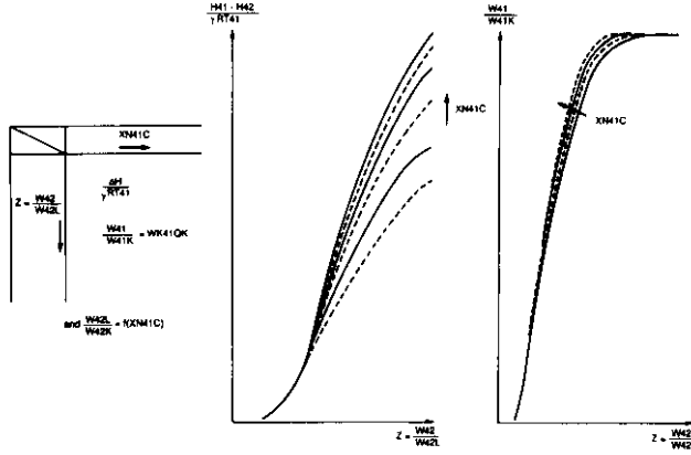
FIGURE 5 - REPRESENTATION OF CHARACTERISTICS OF AN HP TURBINE
