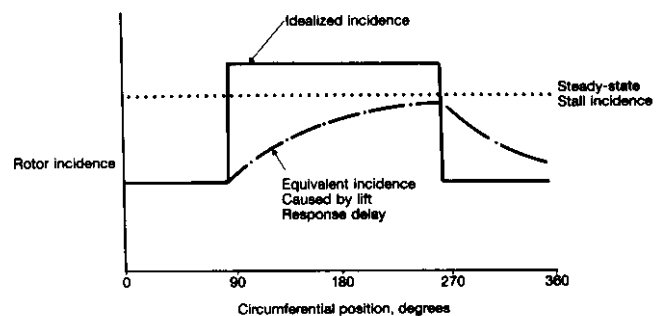
Fig. 17: Effect of Lift Response Delay on Apparent Rotor Stall [8]
