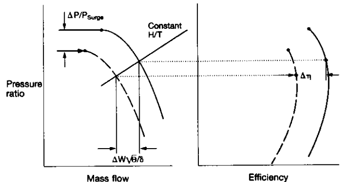
Fig. 14: Reynolds Number Effect on Compressor Performance
