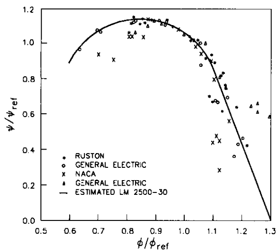
Figure 5 Generalized Stage Pressure Rise Coefficient
