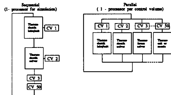
Figure 41 Comparison Between Serial and Parallel Computational Approaches.
