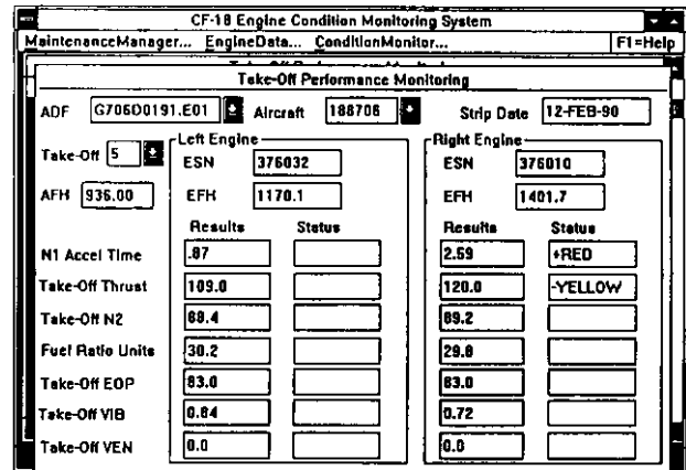
Figure 28-a Typical Diagnostic Output to Operator
