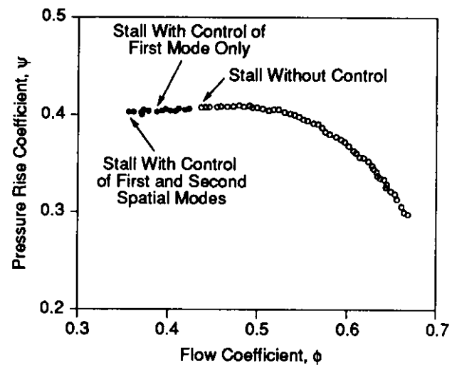
Fig. 28: Compressor characteristic but with active control of first and second spatial modes [21].
