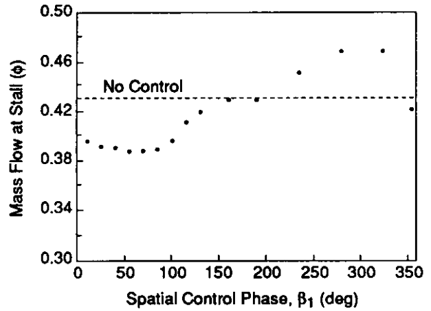
Fig. 26: Influence of feedback control phase angle ( \beta_1 ) on the flow coefficient at which the compressor goes into rotating stall [21].
