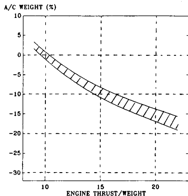
FIG.36 EFFECT OF ENGINE THRUST/WEIGHT ON AIRCRAFT
