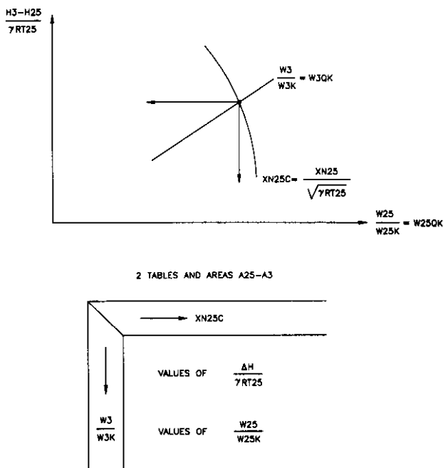
FIGURE 2 - REPRESENTATION OF COMPRESSOR CHARACTERISTICS FOR REFERENCE STATE
