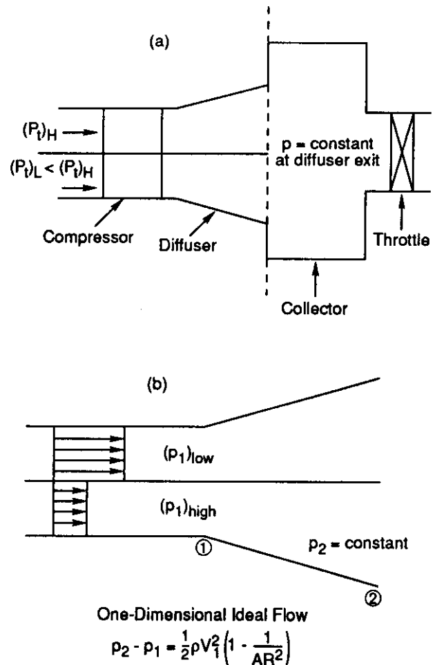
Figure 16: Parallel diffuser model for compressor-component coupling effects; a) parallel diffusers, b) non-uniform flow in a parallel diffuser.
