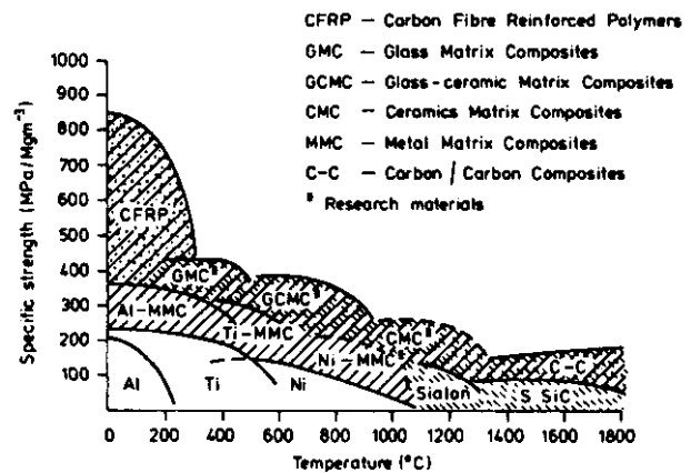
FIG.5 GAS TURBINE MATERIALS (FROM REF 4)
