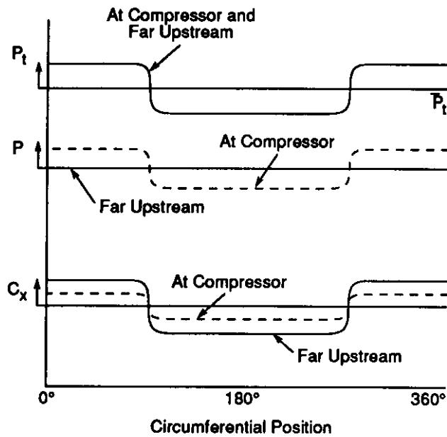
Figure 1: Total pressure, static pressure, and axial velocity distributions at a far upstream station and at the compressor inlet.
