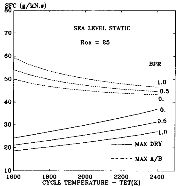
FIG. 29 MILITARY ENGINE SFC TRENDS
