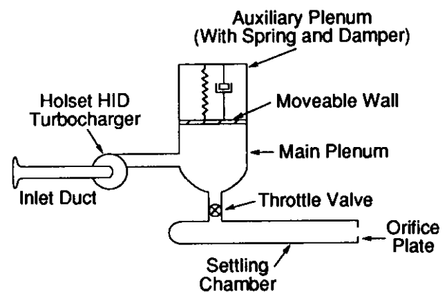
Fig. 11: Schematic of experimental facility for investigation of dynamic structural control.
