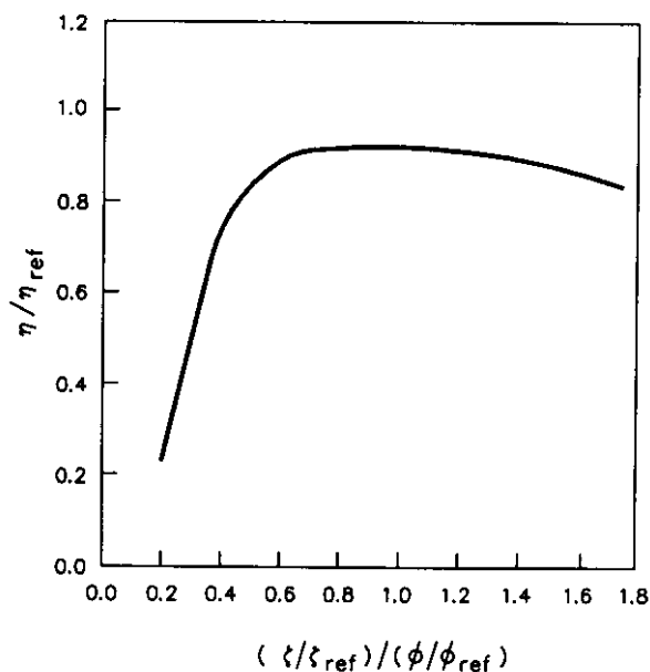
Figure 6 Generalized Stage Efficiency Characteristic
