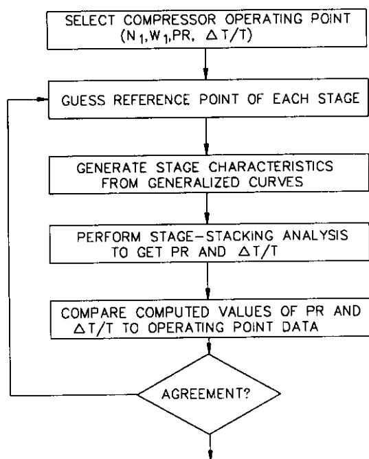
Figure 7 Flowchart for Compressor Characteristic Development
