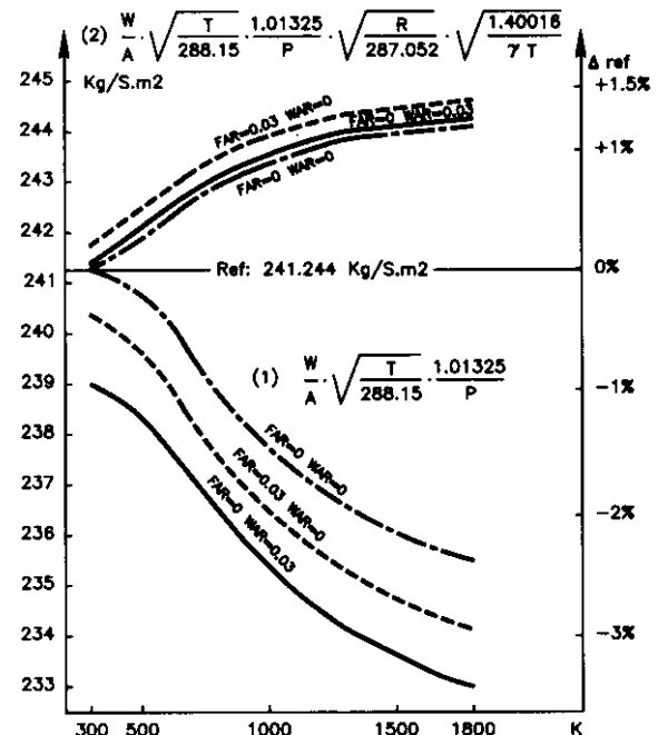
FIGURE 7 - VARIATIONS OF THE CORRECTED MASS FLOW (1) (2) WITH - FLOW TOTAL TEMPERATURE T - WATER (VAPOR) : AIR RATIO WAR - FUEL : AIR RATIO FAR FLOW MACH NUMBER = 1
