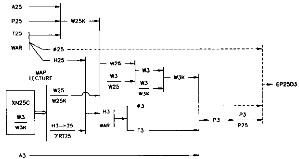
FIGURE 3 - POLYTROPIC EFFICIENCY CALCULATION, USING THE CORRECTED PARAMETERS OF AN HP COMPRESSOR MAP
