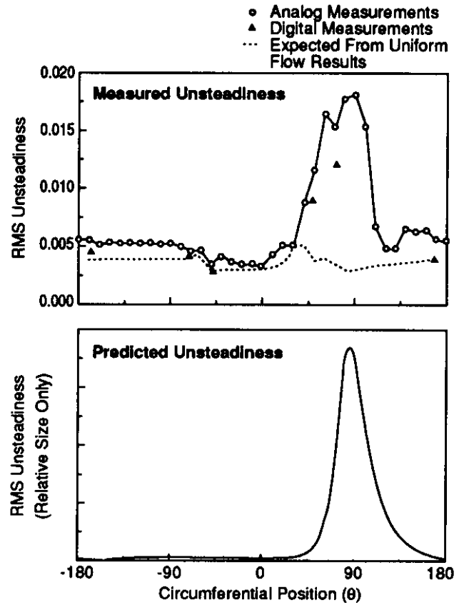
Figure 24: Amplitude of unsteady axial velocity perturbation versus circumferential position for low speed multistage compressor with inlet total pressure distortion [34].
