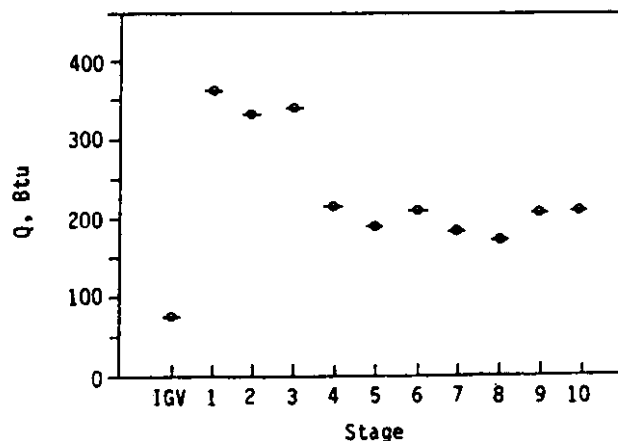
b) Stored thermal energy by stage blading
