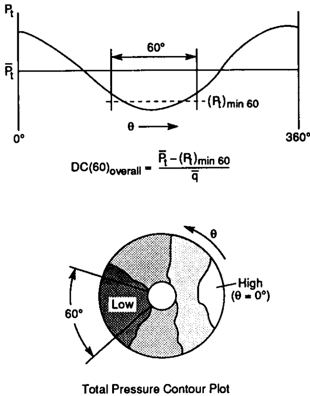
Figure 10: Definition of DC(\theta_{\text{crit}}) parameter for inlet total pressure distortion [10].
