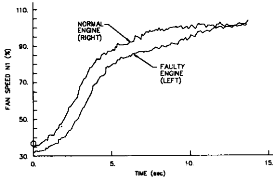
Figure 20 Flight Record of Engine Dynamic Performance with Damaged HP Turbine
