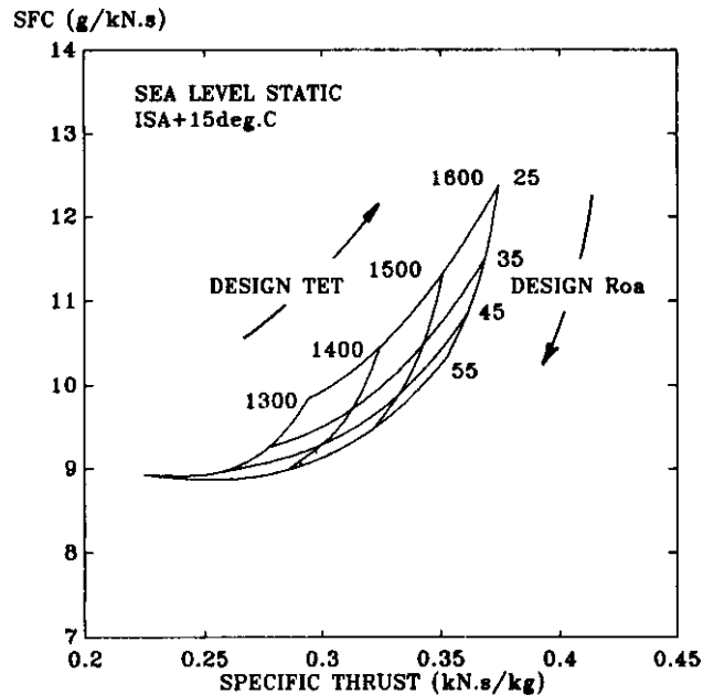
FIG.13 HDTO OFF-DESIGN POINTS - CIVIL ENGINES
