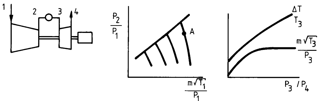
FIG. 7 SINGLE SHAFT
