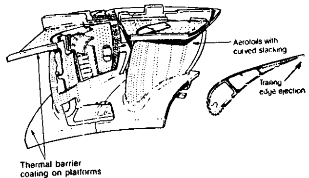
FIG.7 RB211535E4 NOZZLE GUIDE VANE (FROM REF 6)
