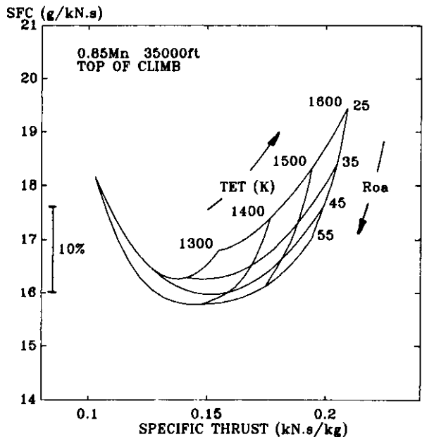
FIG.12 AERODYNAMIC DESIGN POINTS - CIVIL ENGINES
