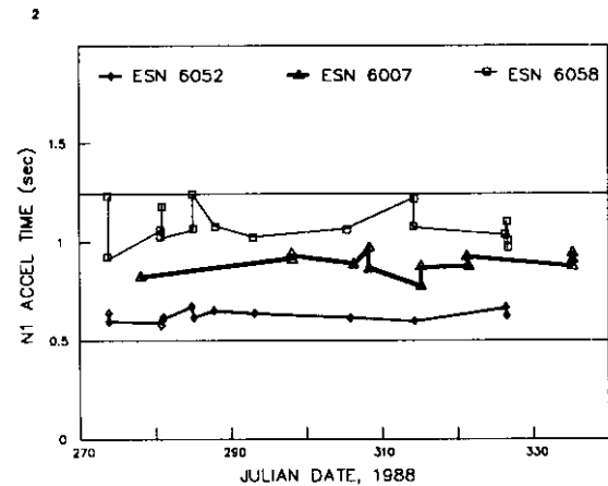
Figure 25 Trend Plots of Different F404-GE-400 Engines
