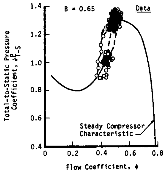
Figure 4 Poststall Behavior of Compressor Rig: Rotating Stall, B = 0.65
