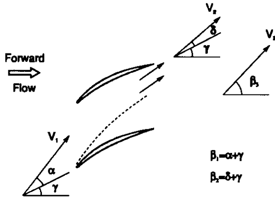
Figure 31 Compressor Cascade Geometry and Nomenclature for Stalled Operation.
