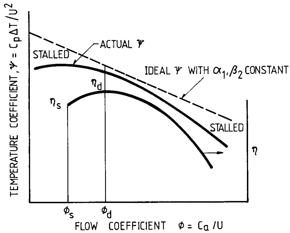
FIG. 5 STAGE CHARACTERISTIC.
