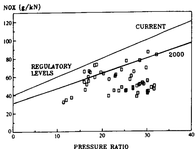
FIG. 23 VARIATION OF NOX WITH CYCLE PRESSURE RATIO
