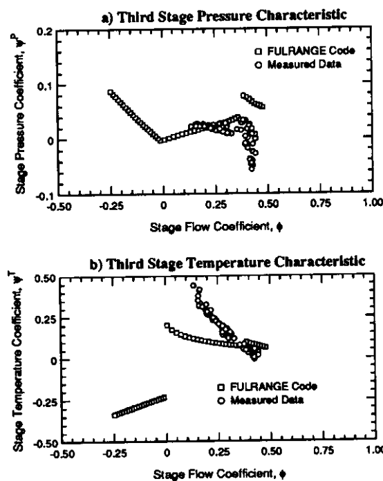
Figure 38 Ten-Stage Compressor: a) Third Stage Pressure Characteristic; b) Third Stage Temperature Characteristic.
