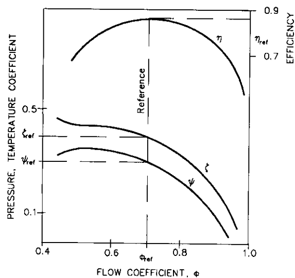
Figure 4 Compressor Stage Characteristics
