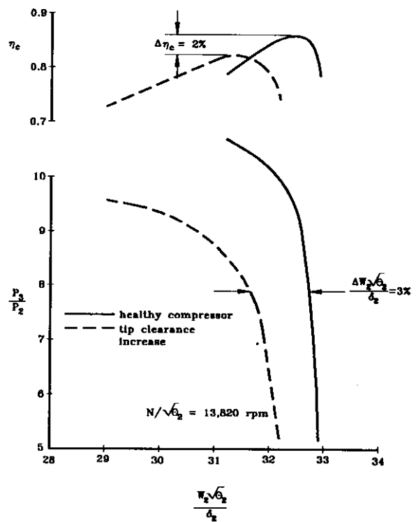
Figure 16 Predicted Influence of Tip Clearance on Axial Compressor Performance
