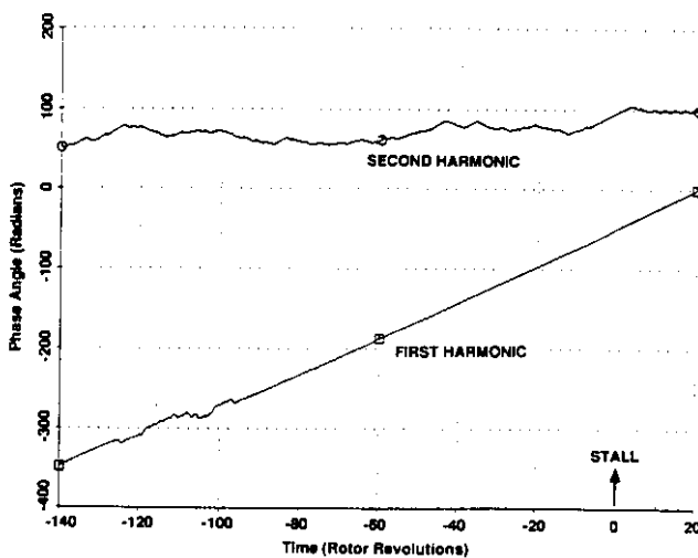
Fig. 19: Time history of the phase of first and second spatial Fourier harmonics measured upstream of a low speed, three-stage compressor [19].
