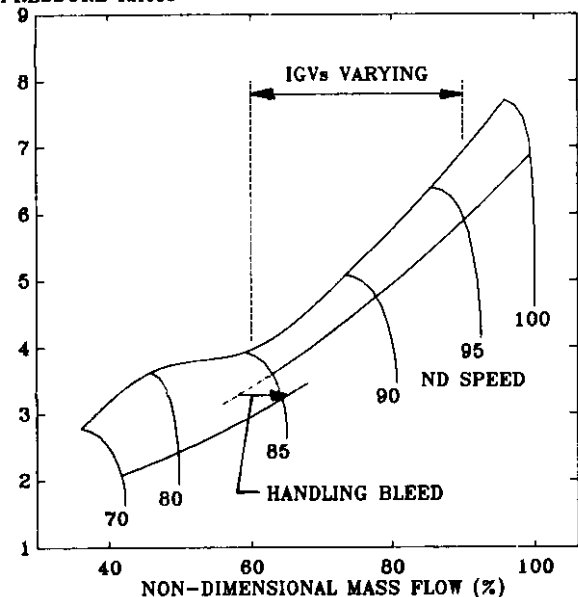
FIG.2 TYPICAL MILITARY HP COMPRESSOR CHARACTERISTIC
