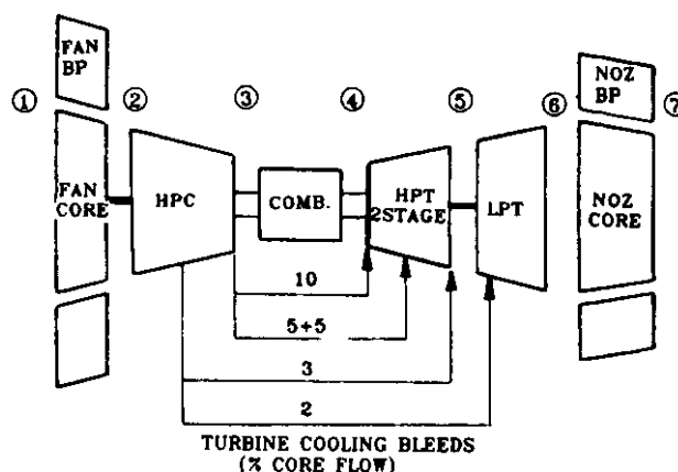
FIG.3 ENGINE CYCLE DIAGRAM (CIVIL TURBOFAN)
