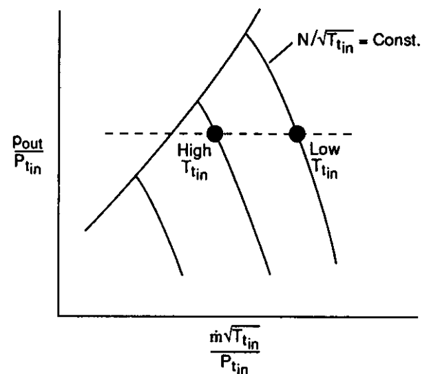
Figure 7: Compressor response to inlet total temperature distortion.
