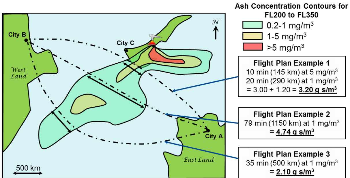
Figure 10: Fabricated example of an ash producing eruption, with ash concentration contours covering the next 6 hours.
