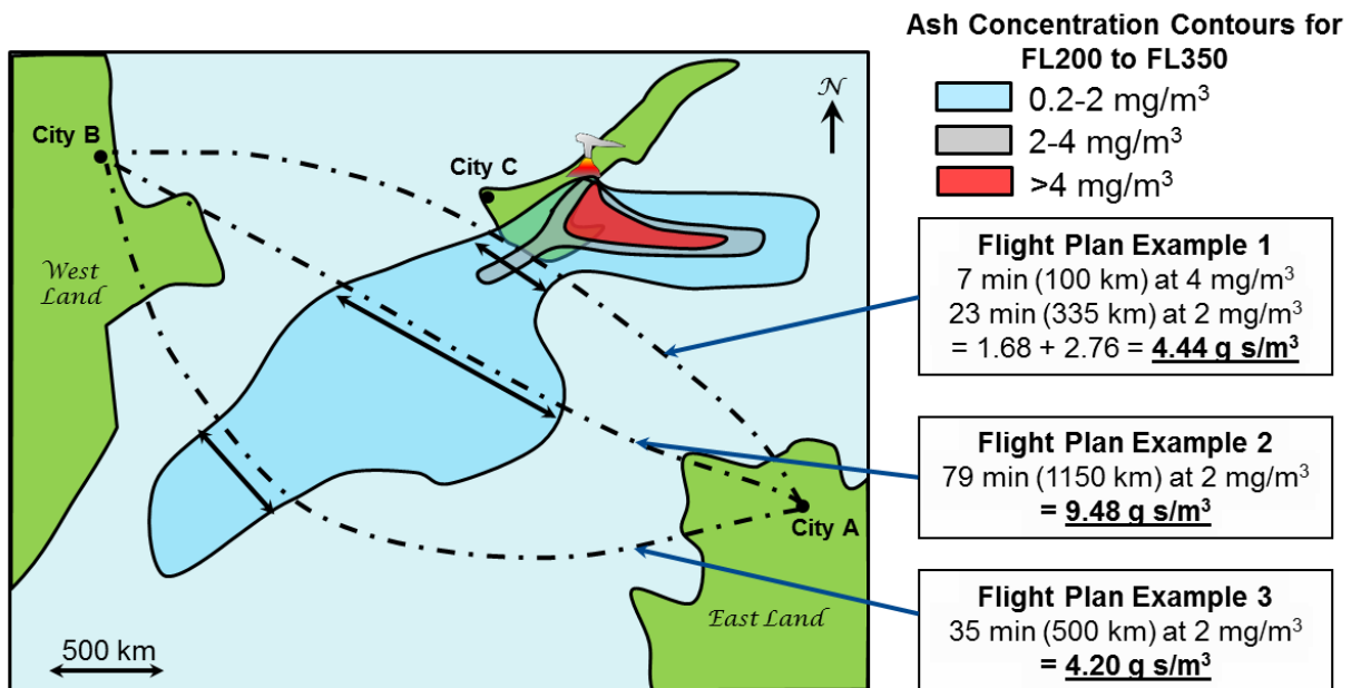
Figure 11: Same ash cloud scenario presented in Figure 10, but with ash contours at 0.2, 2 and 4 \text{ mg}/\text{m}^3 .
