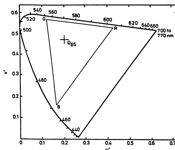
Figure A1.2: The CIE 1976 u' v' diagram with RGB phosphor chromaticities
