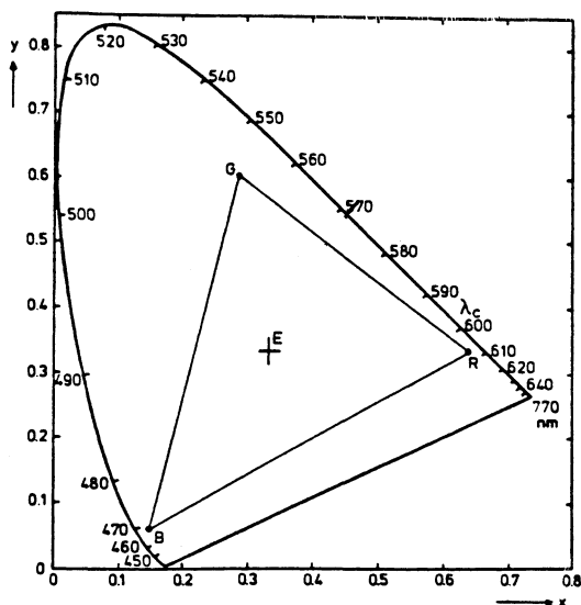
Figure A1.1: The CIE (1931) x,y chromaticity diagram. The chromaticities that can be typically generated on a colour CRT are bounded by the triangle of phosphor chromaticities (R,G,B).
