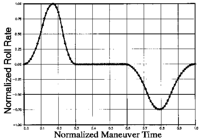
FIG 7: Normalized Roll Rate Trace
