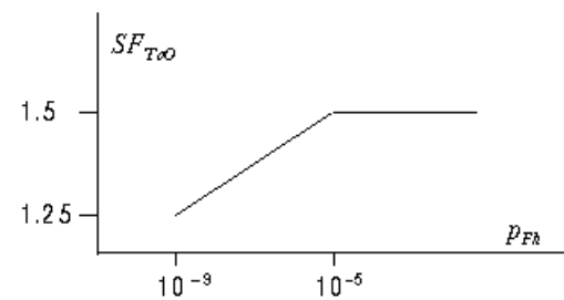
Fig. 1 Safety factor for ToO versus probability of failure per flight hour p_{Fh}
