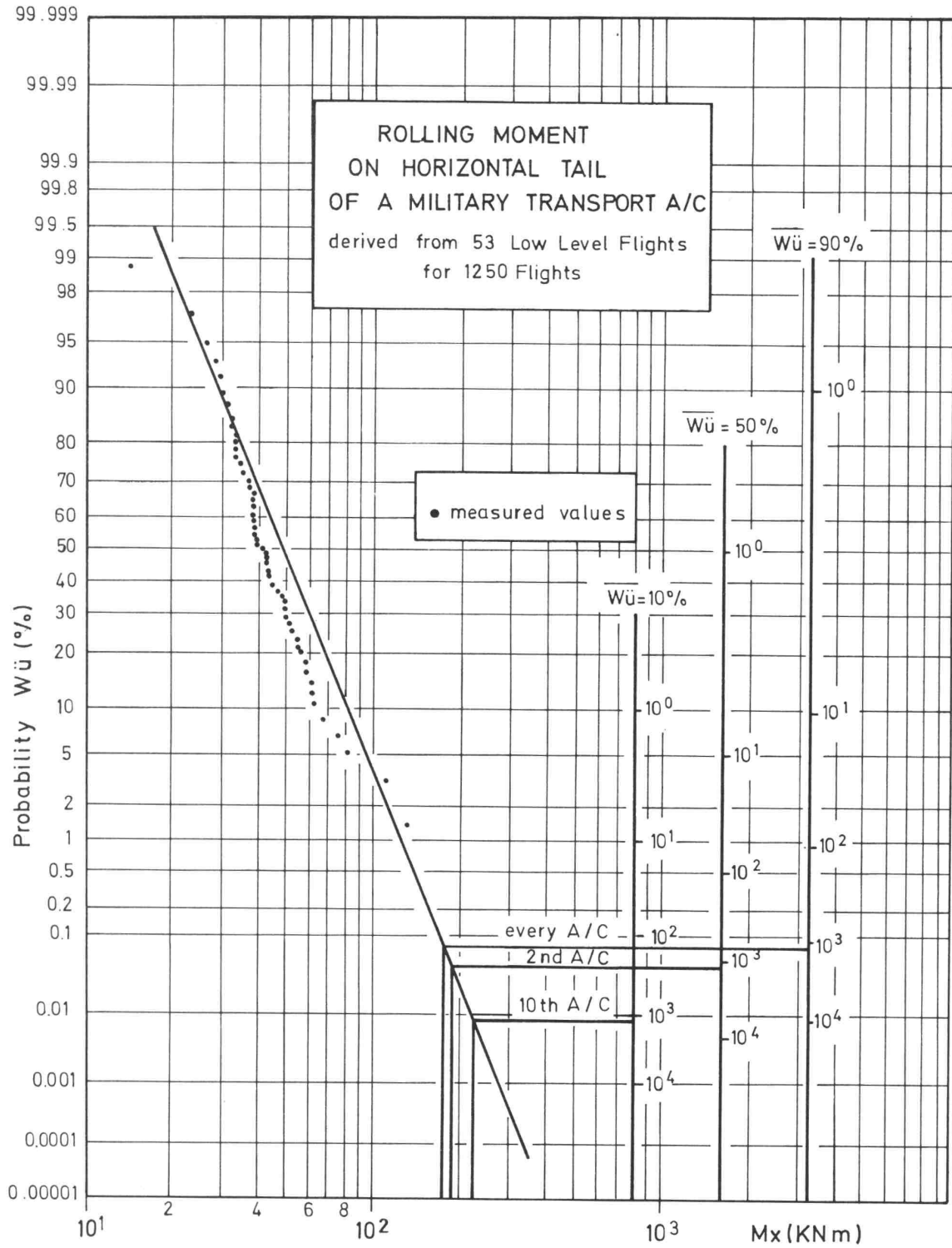
FIG. 1 EXTREME - VALUE DISTRIBUTION
