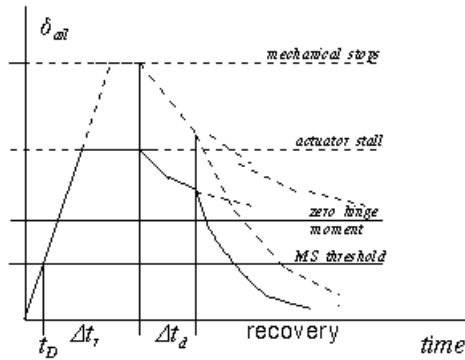
Fig. 5 Supervision of aileron runaway ( \square_{aail} ) detected by MS at t_D , \square_r is runaway time, \square_d is time spent in damping mode
