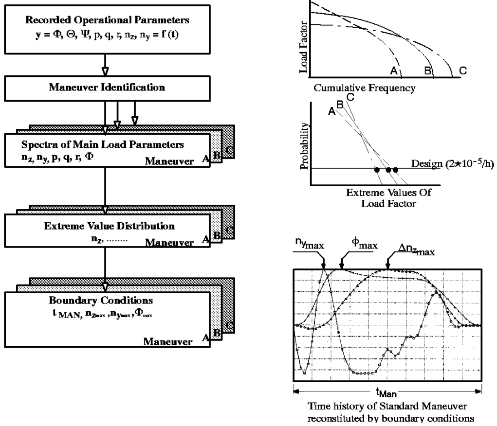
FIG 13 : Boundary Conditions for Design Maneuvers
