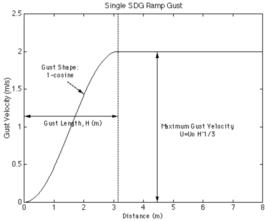
Figure A4.1 Single SDG Gust
