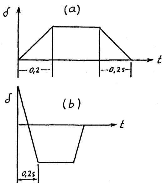
Fig. 5 Rudder Inputs of 8861 A
