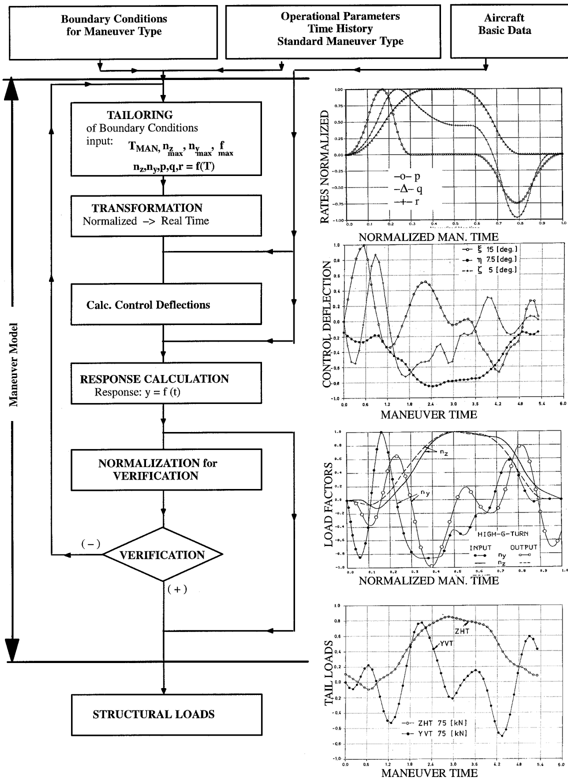
FIG 14 : Procedure of the Operational Maneuver Model
