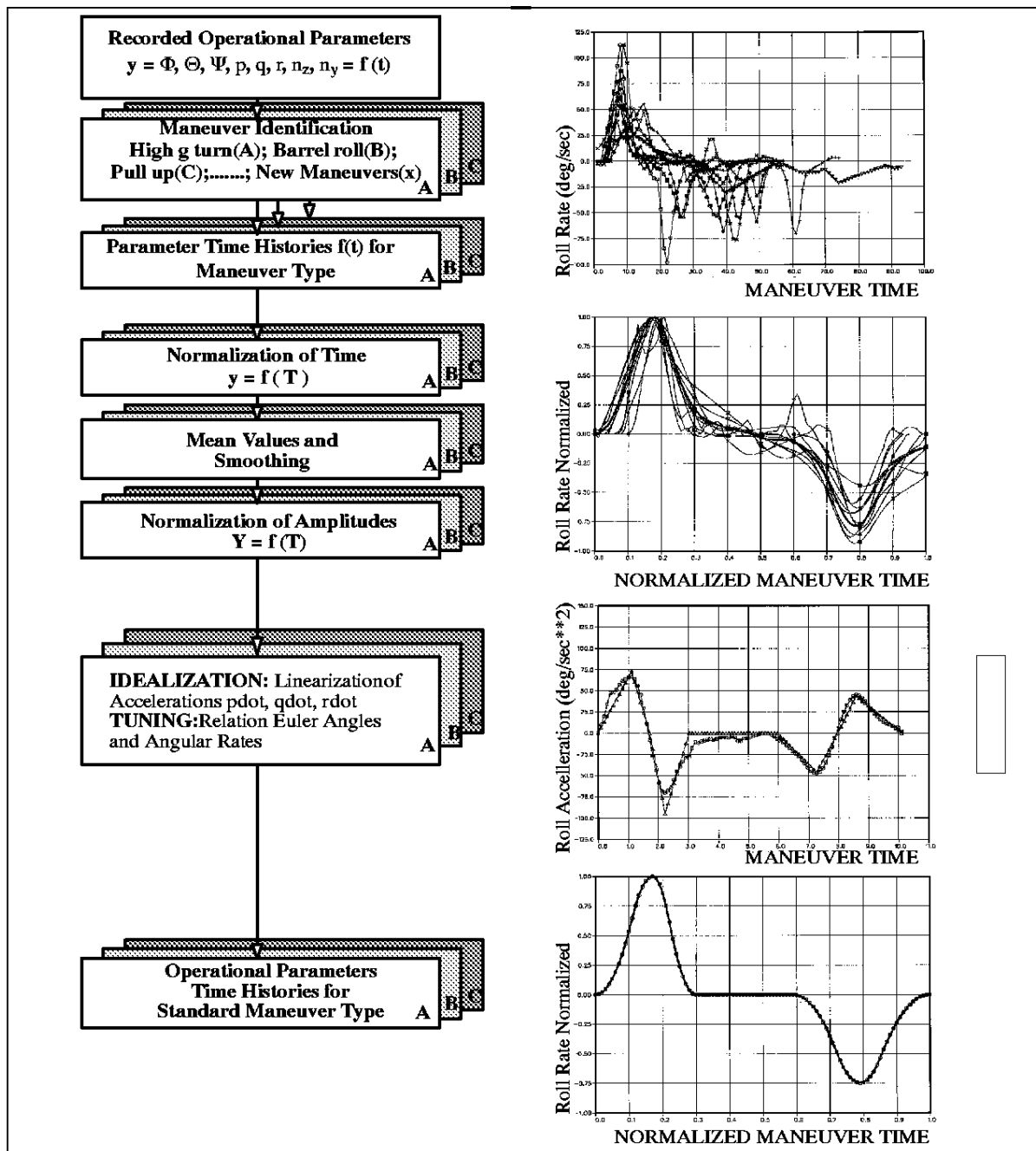
FIG 2: Standard Maneuver Procedure
