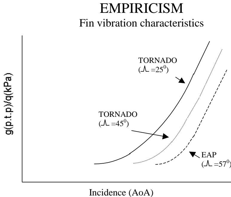
FIGURE 3. Fin Vibration Characteristics
