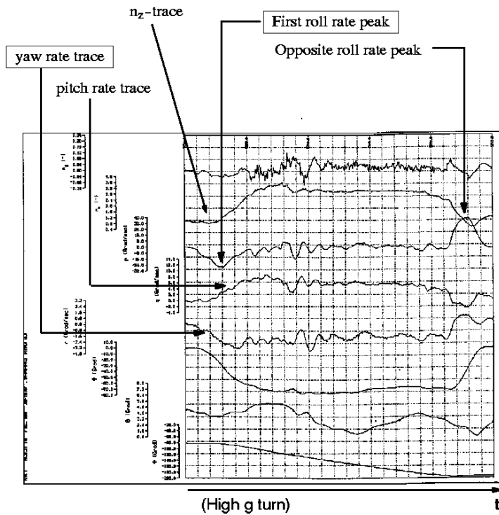
Figure3 :Identified Time Histories of Correlated Operational Parameters
