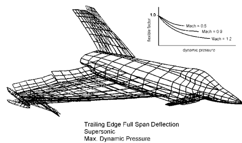
Fig. 12 – Flexible Loads Model - Static Aeroelastic Influences
