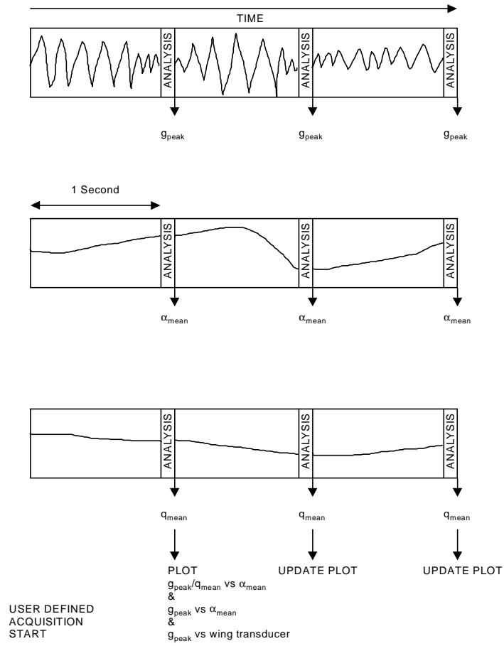
FIGURE 4 - Calculation of Trends With Aircraft Incidence
