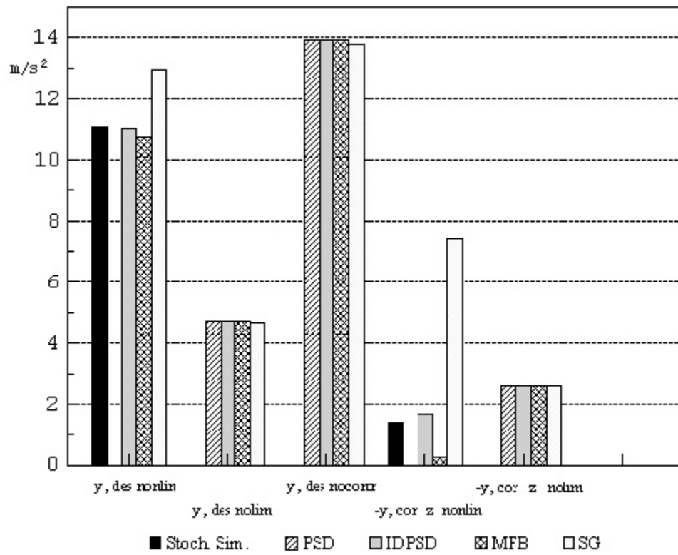
Figure 4.6 Noback Aircraft c/g Acceleration
