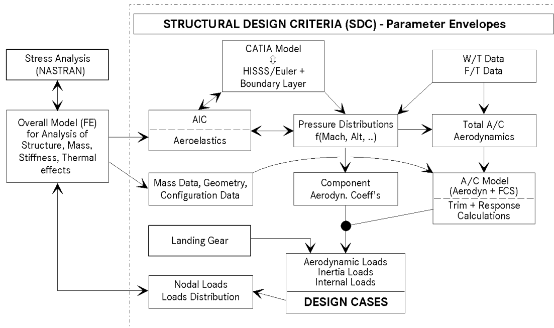
Fig. 3 – Loads Model - Overall View
