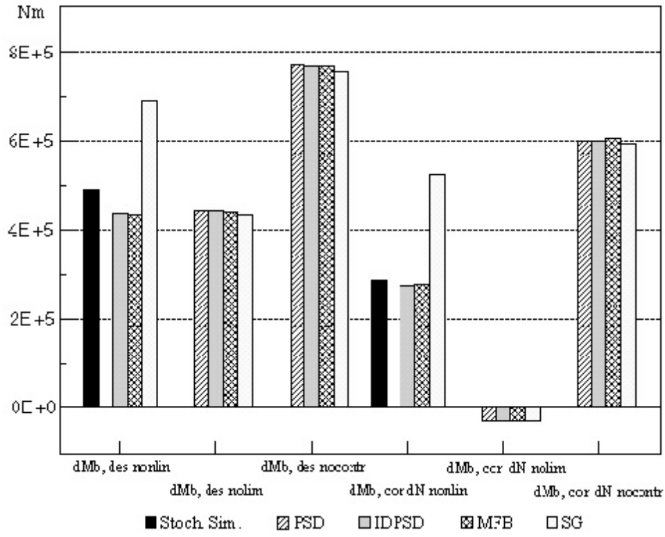
Figure 4.4 F-100 Design and Correlated Loads
