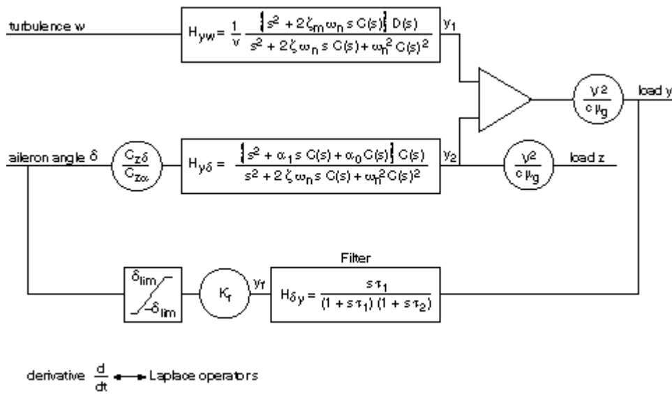
Figure A4.5 Noback Aircraft Model
