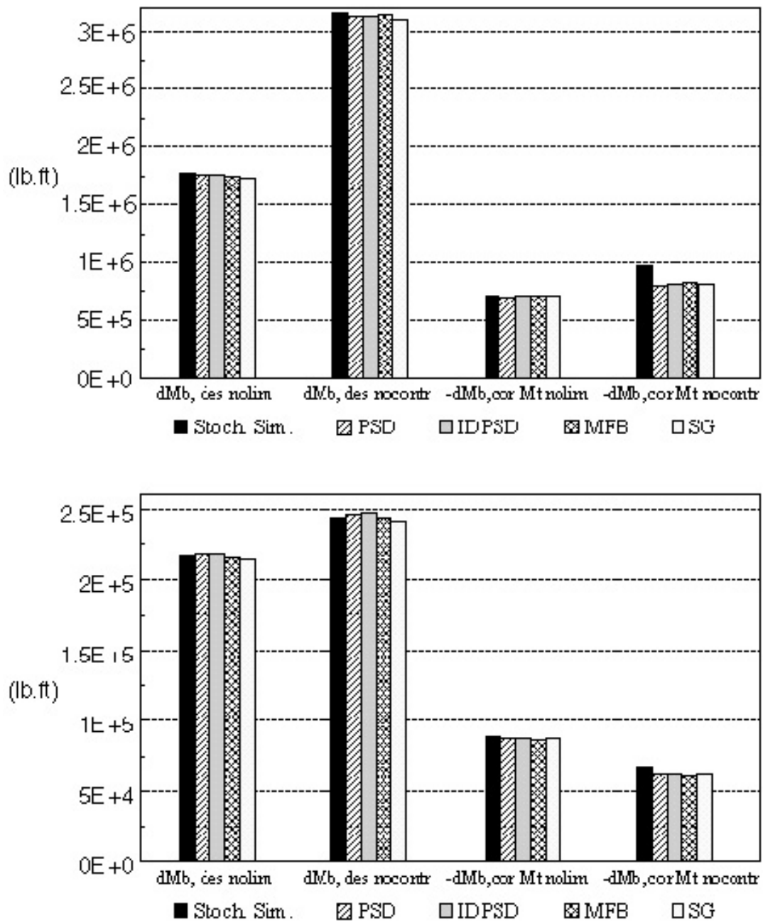
Figure 4.2 Bending and Torsion Loads. Linear A310.
