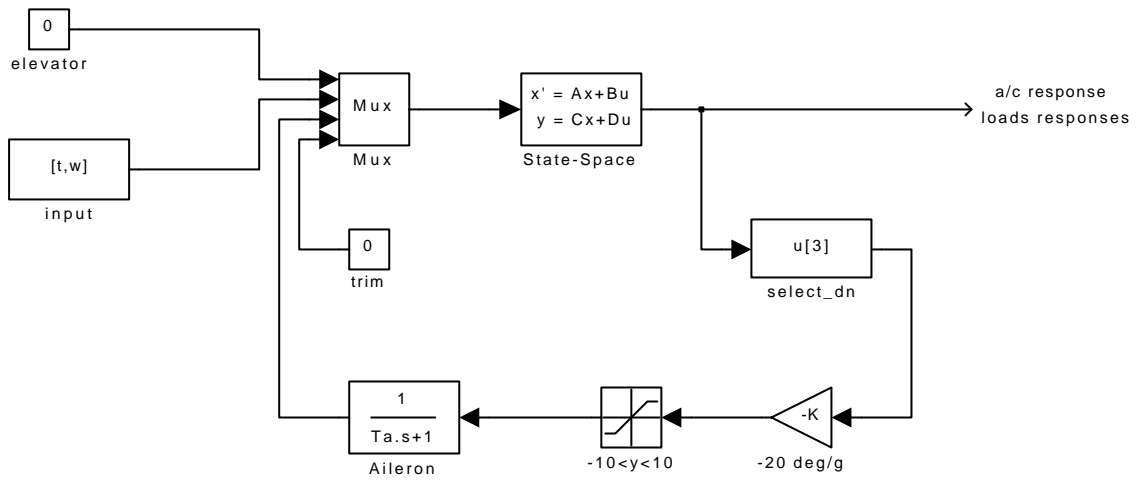
Figure A4.6 Fokker-100 Model
