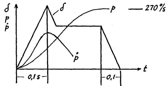
Fig. 4 Stick Input of rolling cases of 8861 A
