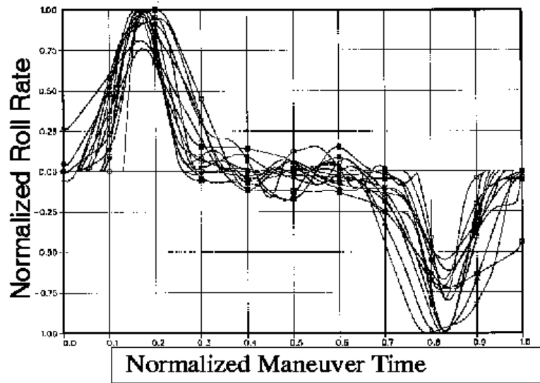
Fig. 10 Comparison of Normalized Rate Traces
