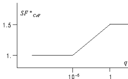
Fig. 2 Contribution to Safety factor for CoF versus probability of being in failure state q = p_{Fh} t_{fail} , the product of p_{Fh} and time spent in failure state t_{fail}
