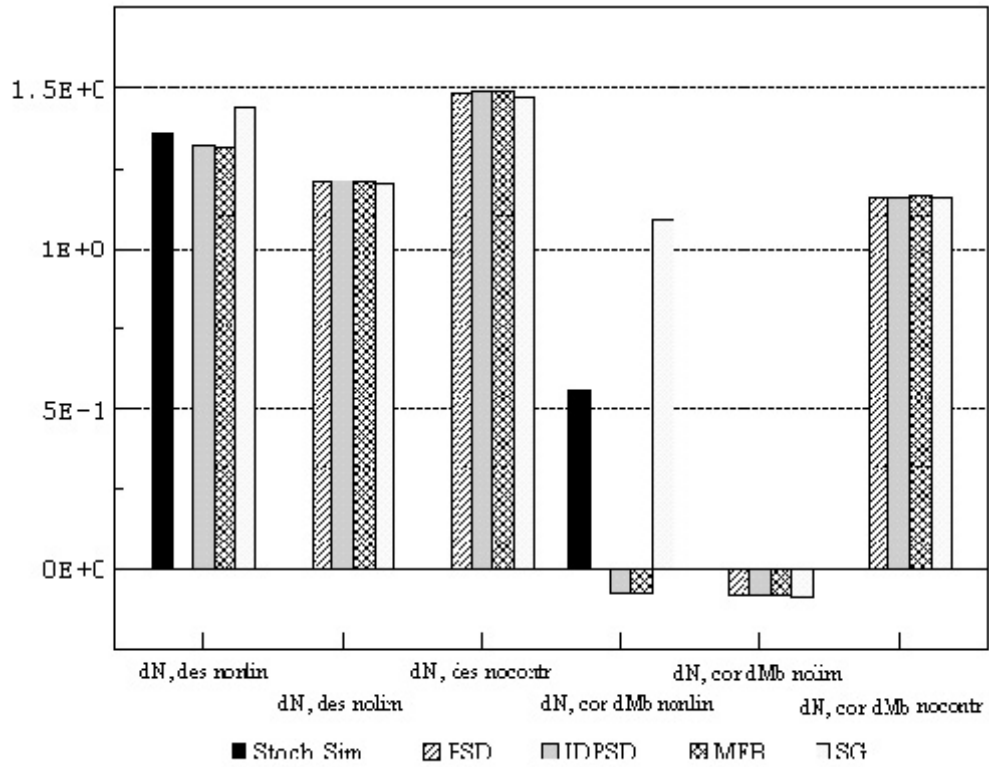
Figure 4.5: F-100 Design and Correlated Loads
