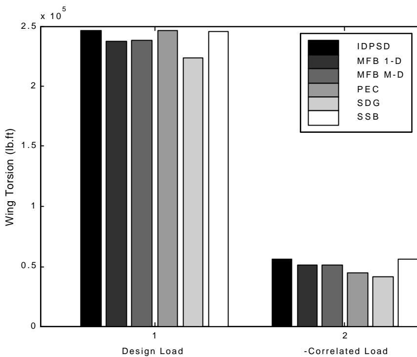
Figure 4.11: Results for A310 model, wing torsion
