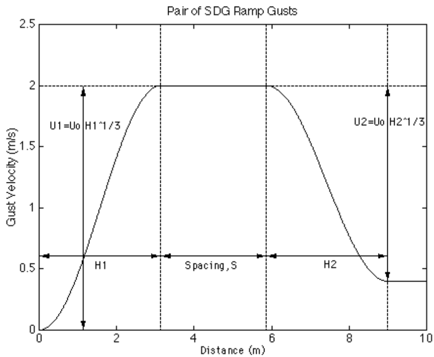
Figure A4.2 Pair of Statistical Discrete Gusts
