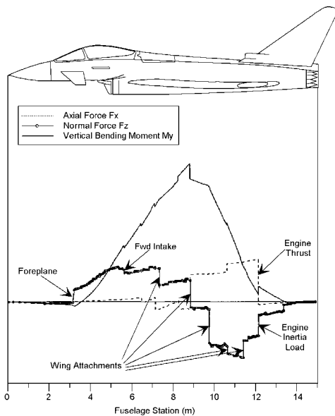
Fig. 4 – Total Aircraft – Balanced Load Case
