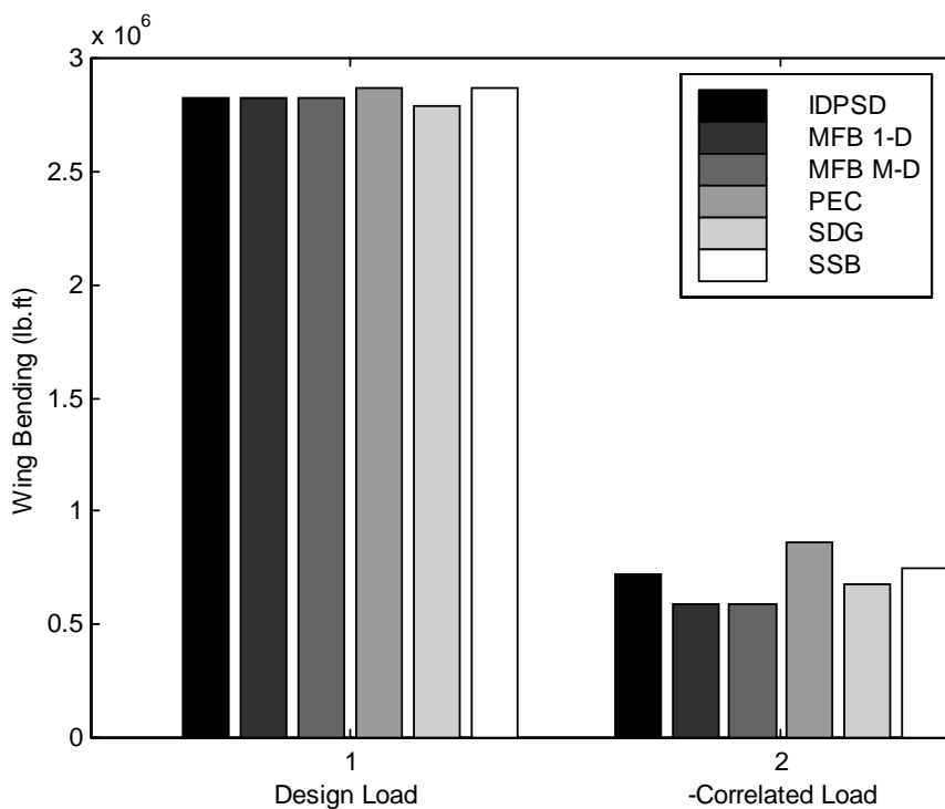
Figure 4.10: Results for A310 model, wing bending
