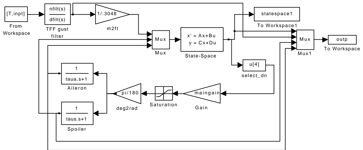
Figure A4.7 A310 Model
