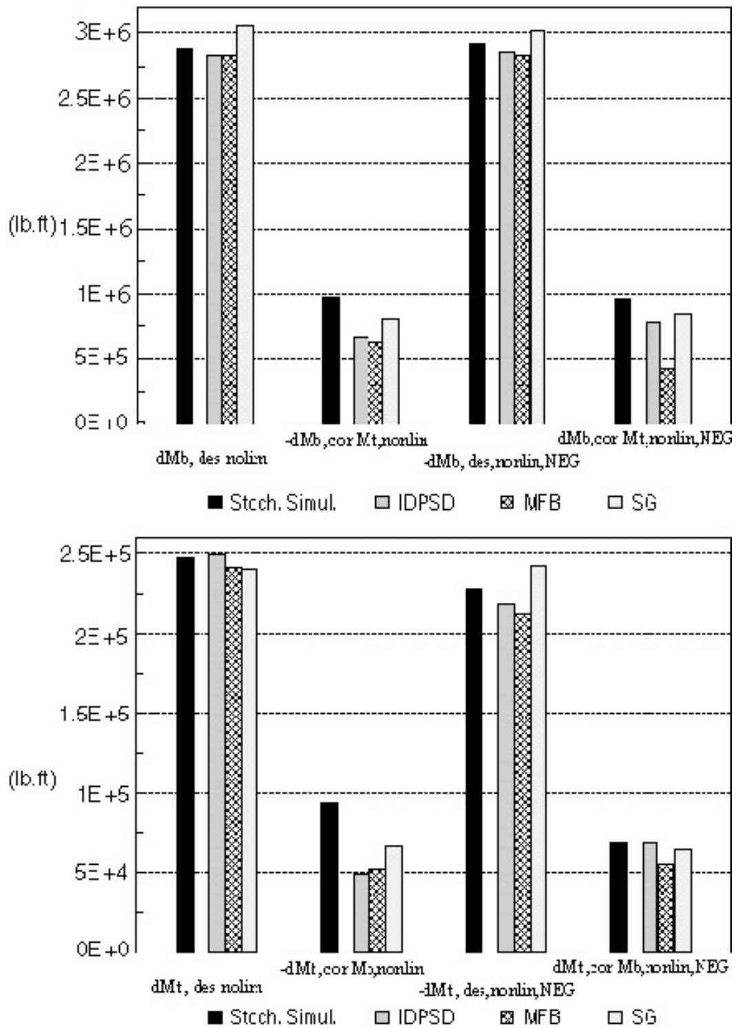
Figure 4.3 Bending and Torsion Loads. Non-Linear A310.
