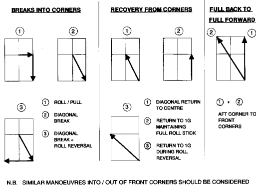
Fig. 7 – Typical Pilot Stick Input
