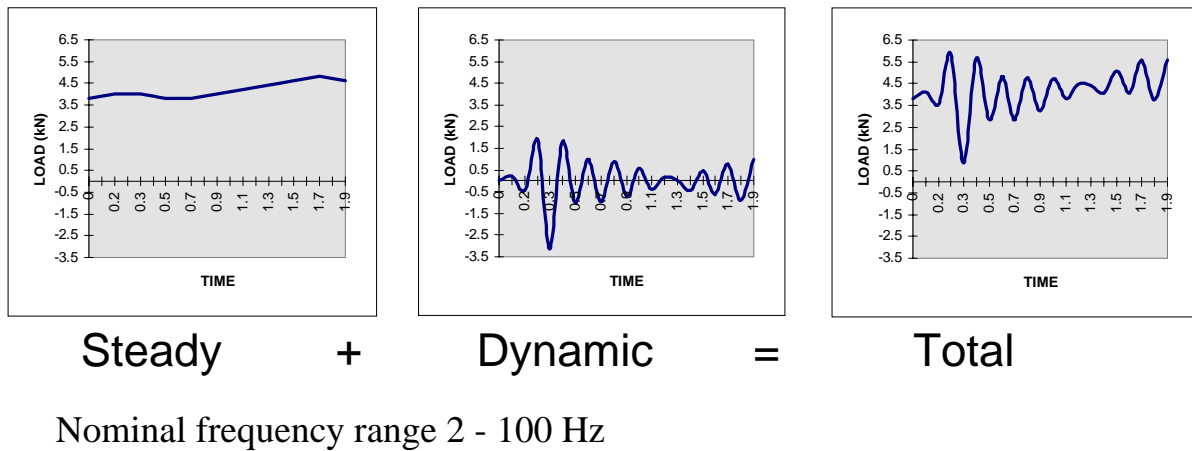
Figure 6: Superposition of Steady and Unsteady Loads
