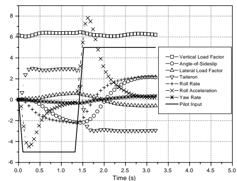
Fig. 6 – MIL - Rolling Pull Out Maneuver
