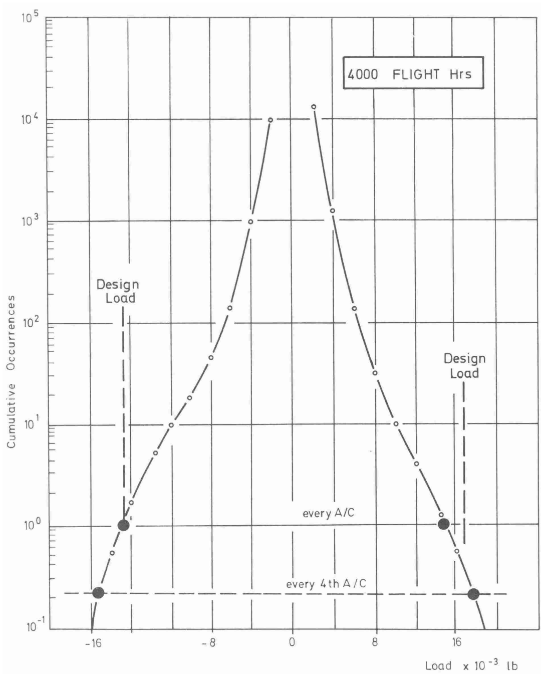
FIG. 2 CUMULATIVE OCCURRANCES OF VERTICAL STABILIZER LOADS
