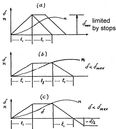
Fig. 2 Stick Inputs for pitching cases of 8861A
