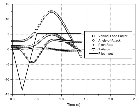
Fig. 5 – MIL - Pull-Push Maneuver
