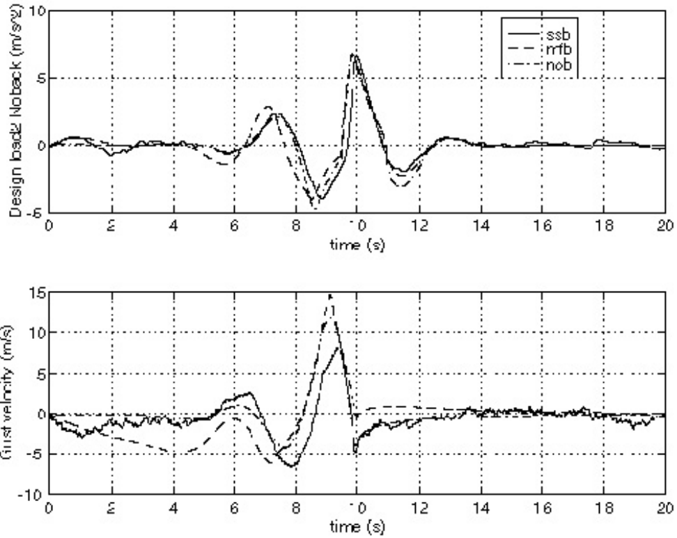
Figure 4.12: Comparison between SSB, MFB 1-D and IDPSD (labeled 'nob') for Noback a/c load 2 (design load and gust shape)
