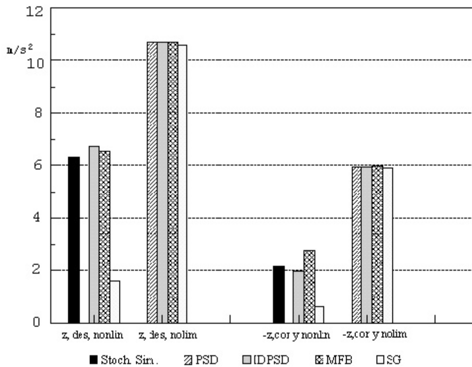
Figure 4.7 Noback Model c/g Acceleration by Aileron
