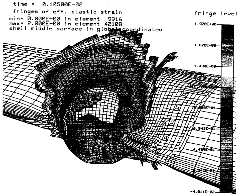
Figure 6: Birdstrike FE-Prediction
