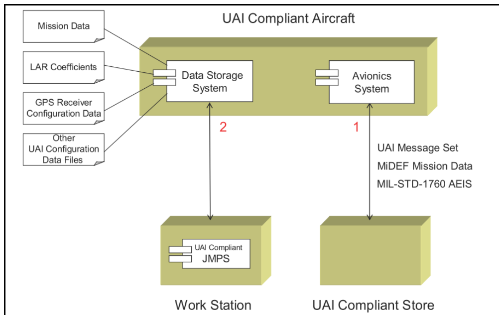
Figure 7-1: UAI System Interface Description.
